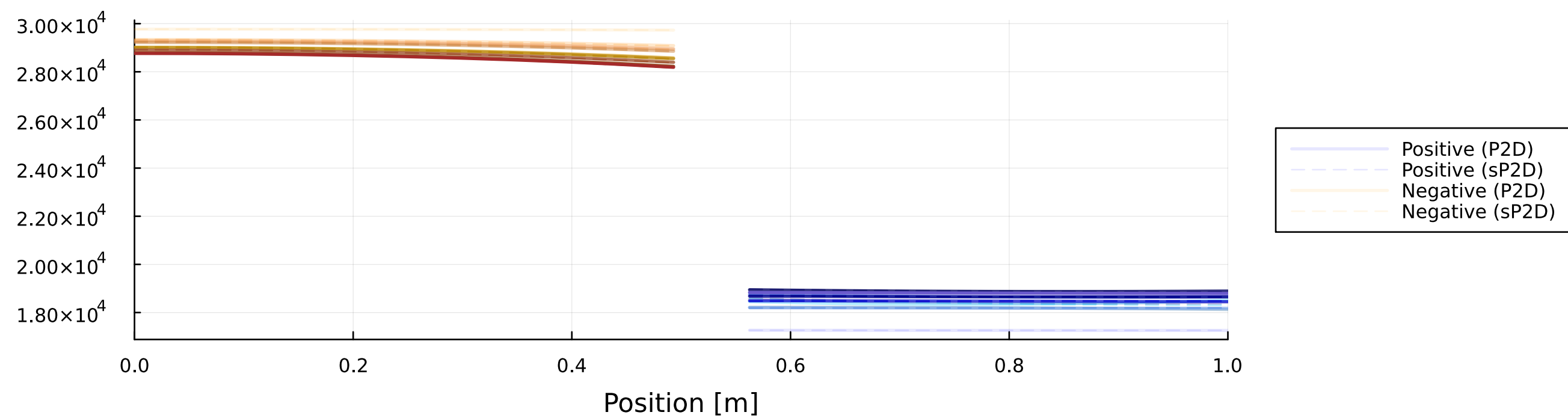
Electrode Stress Distribution (P2D &amp; sP2D) - UDDS
